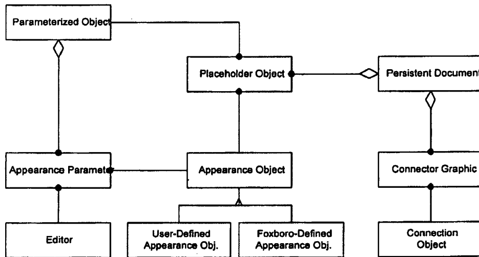
Figure 29B - Combined Placeholder/Appearance Object Model
